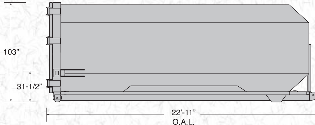
SIDE ELEVATION
